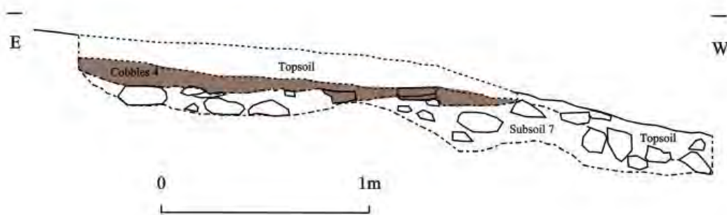
Figure 1 Section 39 E-W, across Trench 6 2m from S end showing the cobbled layer (partly excavated)
